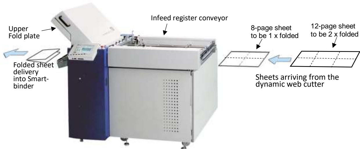
F-100 cross-folder unit used directly before SB infeed
